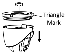
Figure 2-35 Disassemble the Camera
