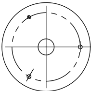
Figure 2-38 Drill Template
