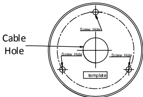
Figure 2-1 Drill Template
